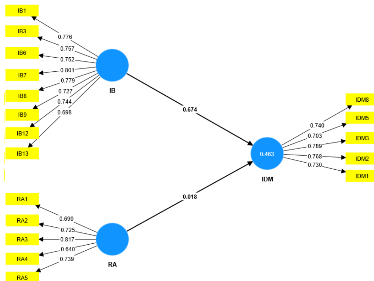
Fig. 2. Measurement Model
