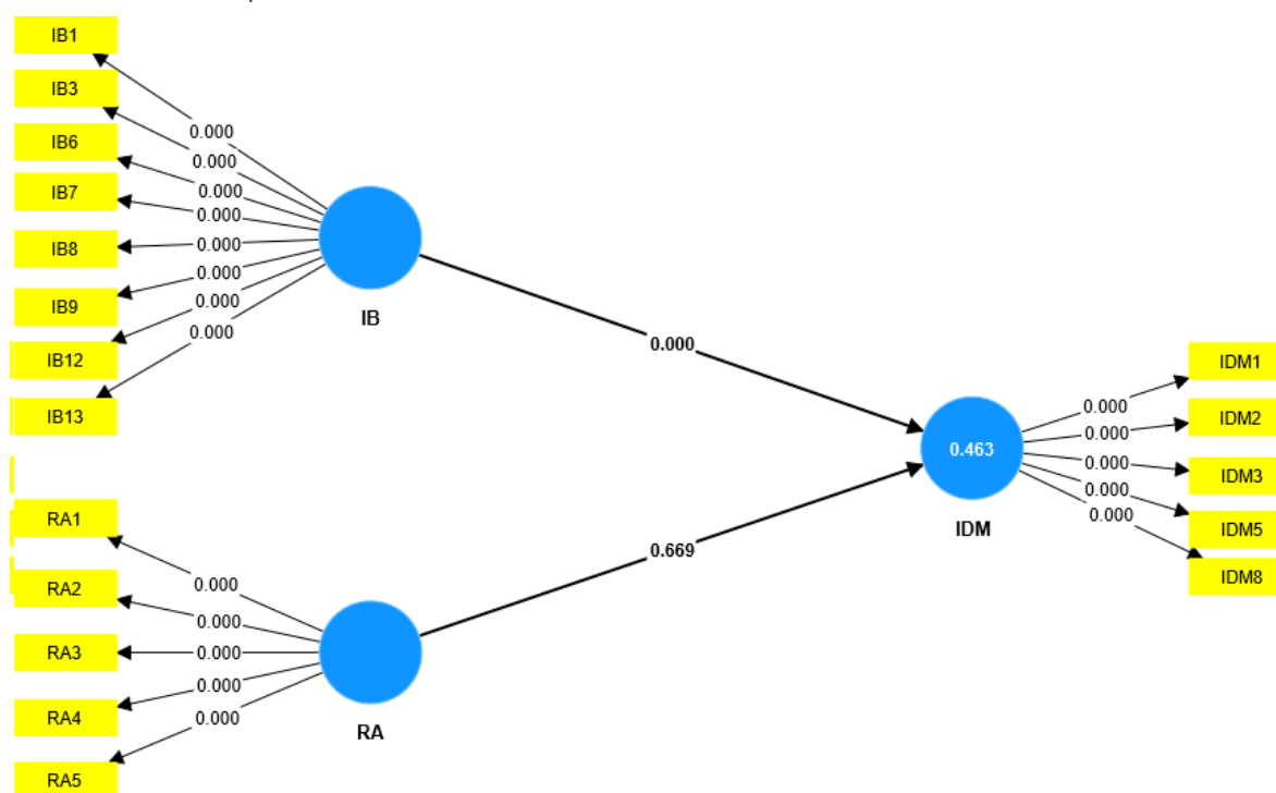
Fig. 3. Structural Model
